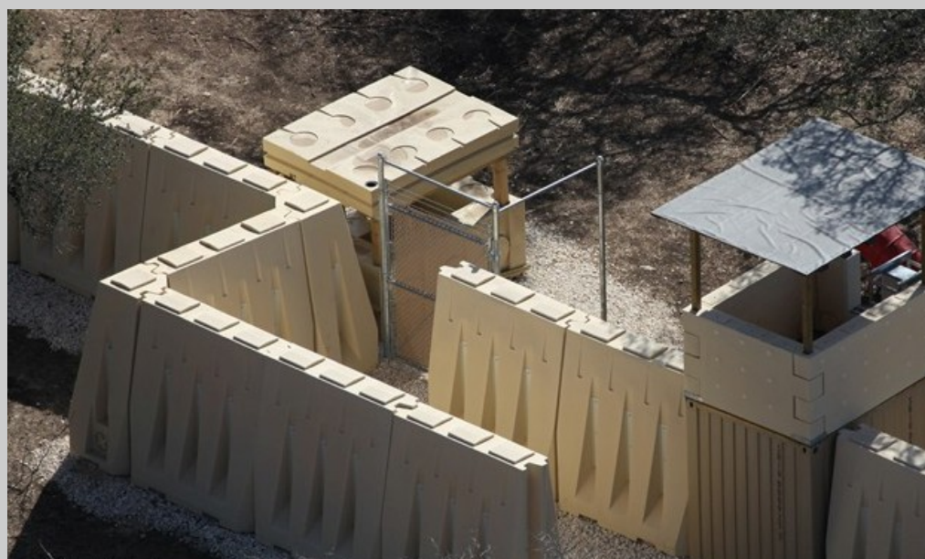
Check Point bunker as part of a ECP
